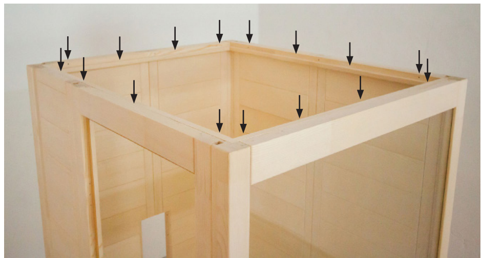
16 screws: 3.5 x 50 mm
