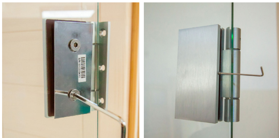
Fig. 32: Installing door fittings 2
