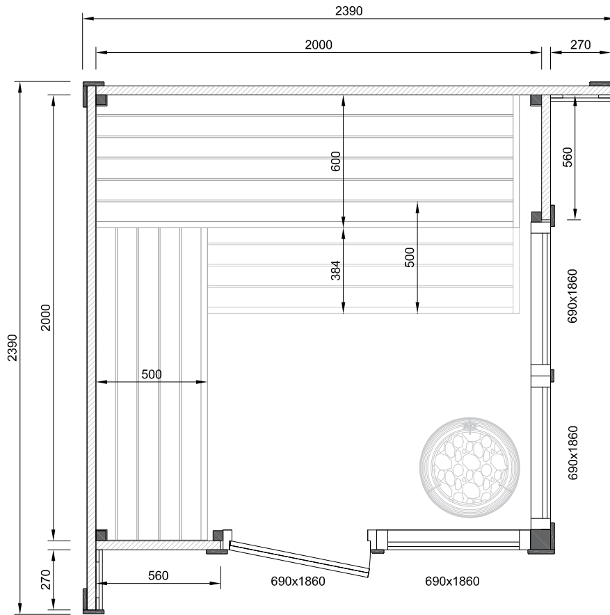
Layout
