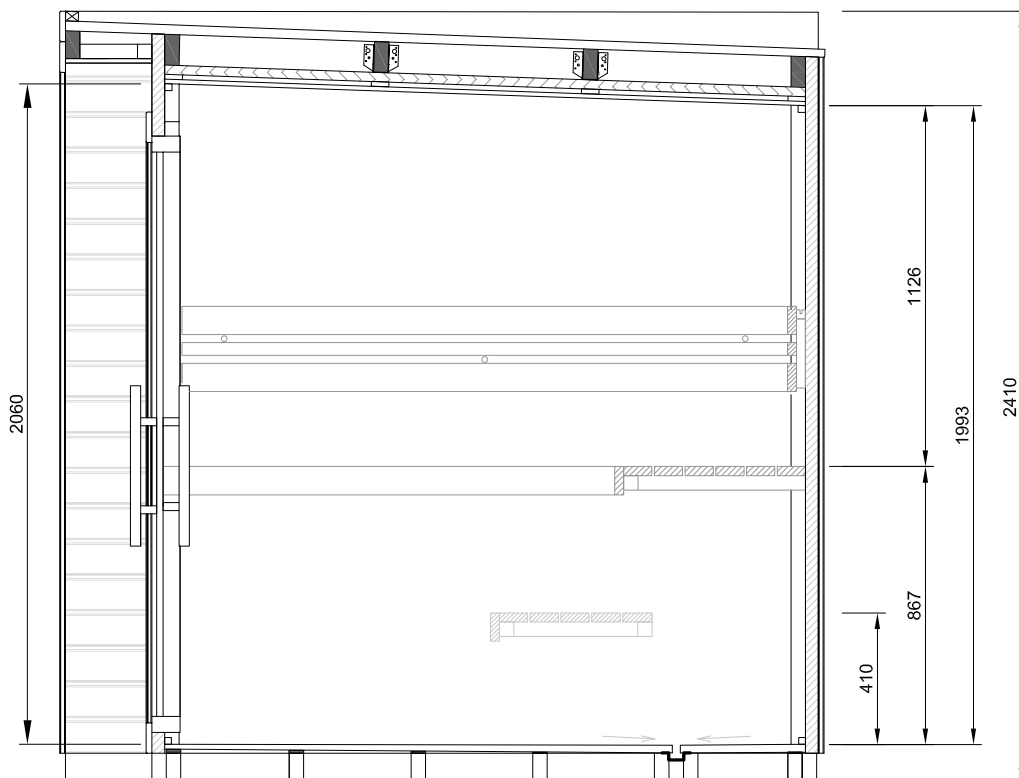
Cross section
